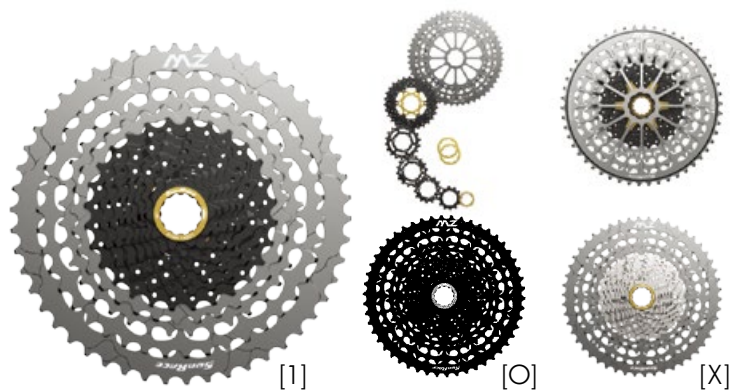
CSMZX1 WT5 10-50T [12-Speed Wide Ratio] [A7075 CNC 32~50T Sprocket] [Alloy Spiders] [Alloy Lockring & Spacers] 1 [Black Chrome + Gray] O [Black Chrome + Black] X [Metallic Silver + Gray] 462g
