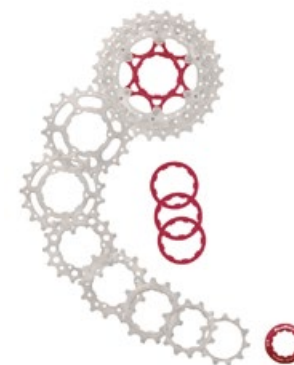
[10-Speed] [Alloy Spider] [Alloy Spacer] [Alloy Lockring] O[Black Chrome] / X[Metallic Silver] 236g[AQ] / 245g[AS] 304g[AU] / 320g[AV] / 290g [BS]
