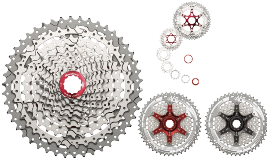
CSMX3 TAZ 11-46T TAY 11-42T TAX 11-40T [10-Speed Wide Ratio] [A7075 Largest Sprocket] [Alloy Spiders] [Alloy Lockring & Spacers] O[Black Chrome] / X[Metallic Silver] 436[AZ] / 393g[AY] / 385g[AX]
