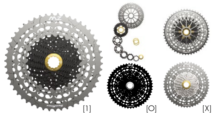
CSMZX0 WA5 11-50T [12-Speed Wide Ratio] [A7075 CNC 32~50T Sprocket] [Alloy Spiders] [Alloy Lockring & Spacers] 1 [Black Chrome + Gray] O [Black Chrome + Black] X [Metallic Silver + Gray] 469g
